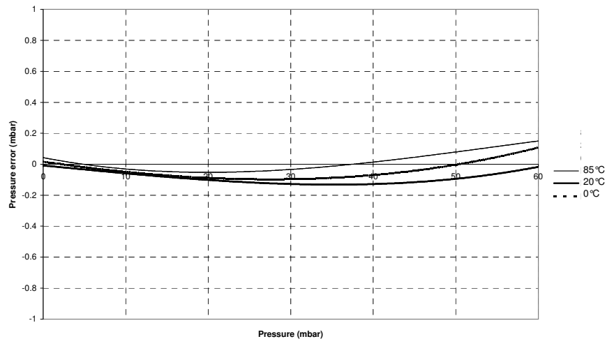
Absolute Pressure Accuracy after Calibration
